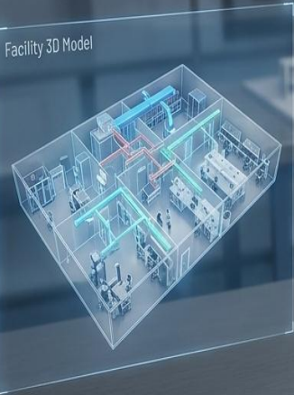
3D Cleanroom airflow
